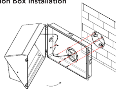
Junction Box Installation
