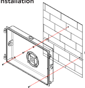
Direct Wall-Mount Installation
