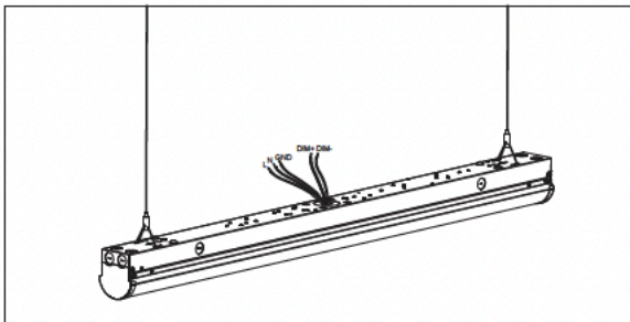
3. Connect the AC wires and dimming wires.
