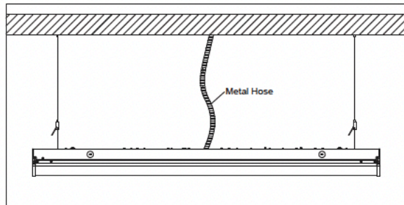
4. Wrap the wires with metal conduit.
